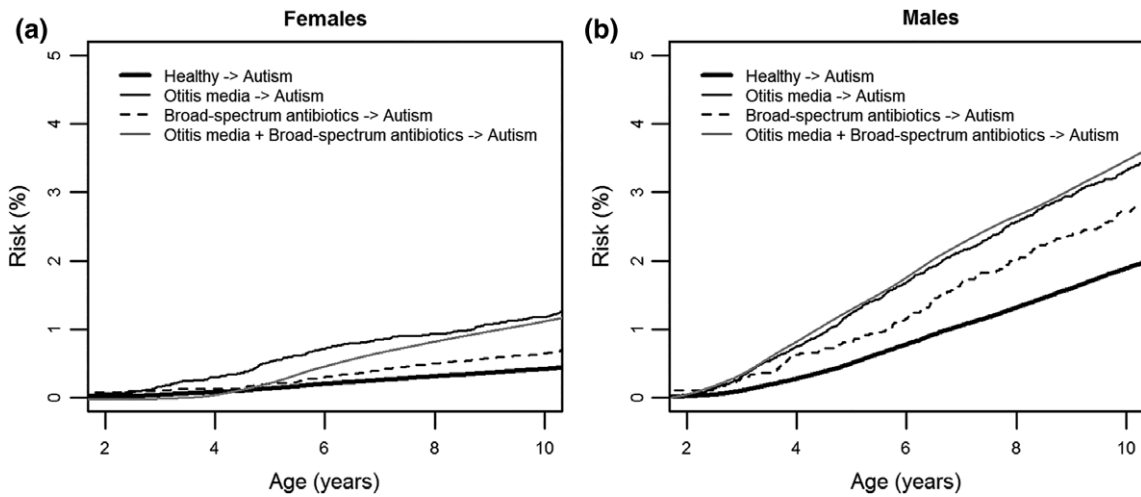
Figure 2. Absolute risk of autism for females (A) and males (B). The risk of transitioning from [otitis media + broad-spectrum antibiotics] → [autism] was smoothed to avoid potential identification of individuals.
